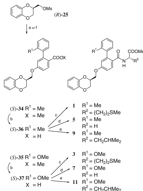
Scheme 2. Synthesis of compounds 1, 5, 9, 3, 7 and 11 : (a) 32 , NaH, DME, –20 °C and then reflux, 72 h, 69%; (b) 3 N KOH, acetone, 50 °C, 12 h, 80% (( S )- 36 ) and 76% (( S )- 37 ); (c) L-methionine methyl ester hydrochloride, HOBt, EDAC, DMF, 15 min, room temperature and then TEA, 24 h, room temperature, 90% ( 1 ) and 94% ( 3 ); (d) glycine methyl ester hydrochloride, HOBt, EDAC, DMF, 15 min, room temperature and then TEA, 24 h, room temperature, 88% ( 5 ) and 69% ( 7 ); (e) L-leucine methyl ester hydrochloride, HOBt, EDAC, DMF, 15 min, room temperature and then TEA, 24 h, room temperature, 90% ( 9 ) and 85% ( 11 ); (f) 33 , NaH, DME, –20 °C and then reflux, 72 h, 74%.
